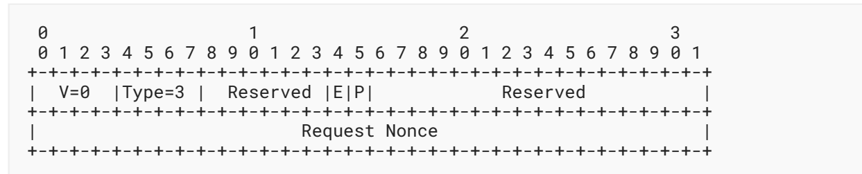
Figure 2: Updated AMT Request Message Format
