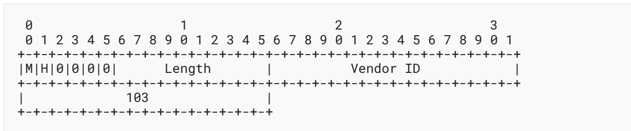
Figure 1: ECN Capability AVP for L2TP (v2 or v3)
