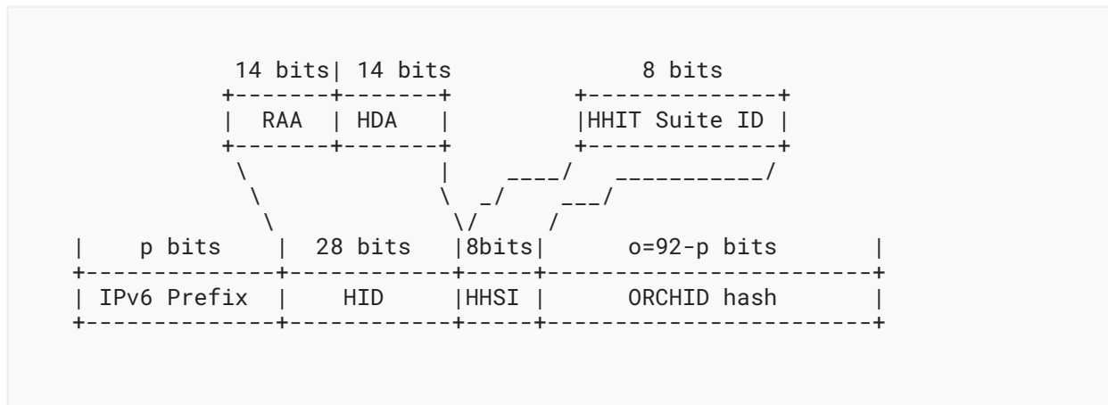
Figure 1: HHIT Format
